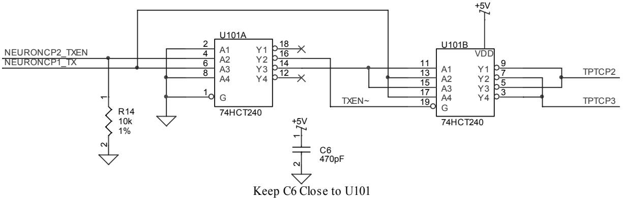
Figure 2. Differential Driver Circuit
