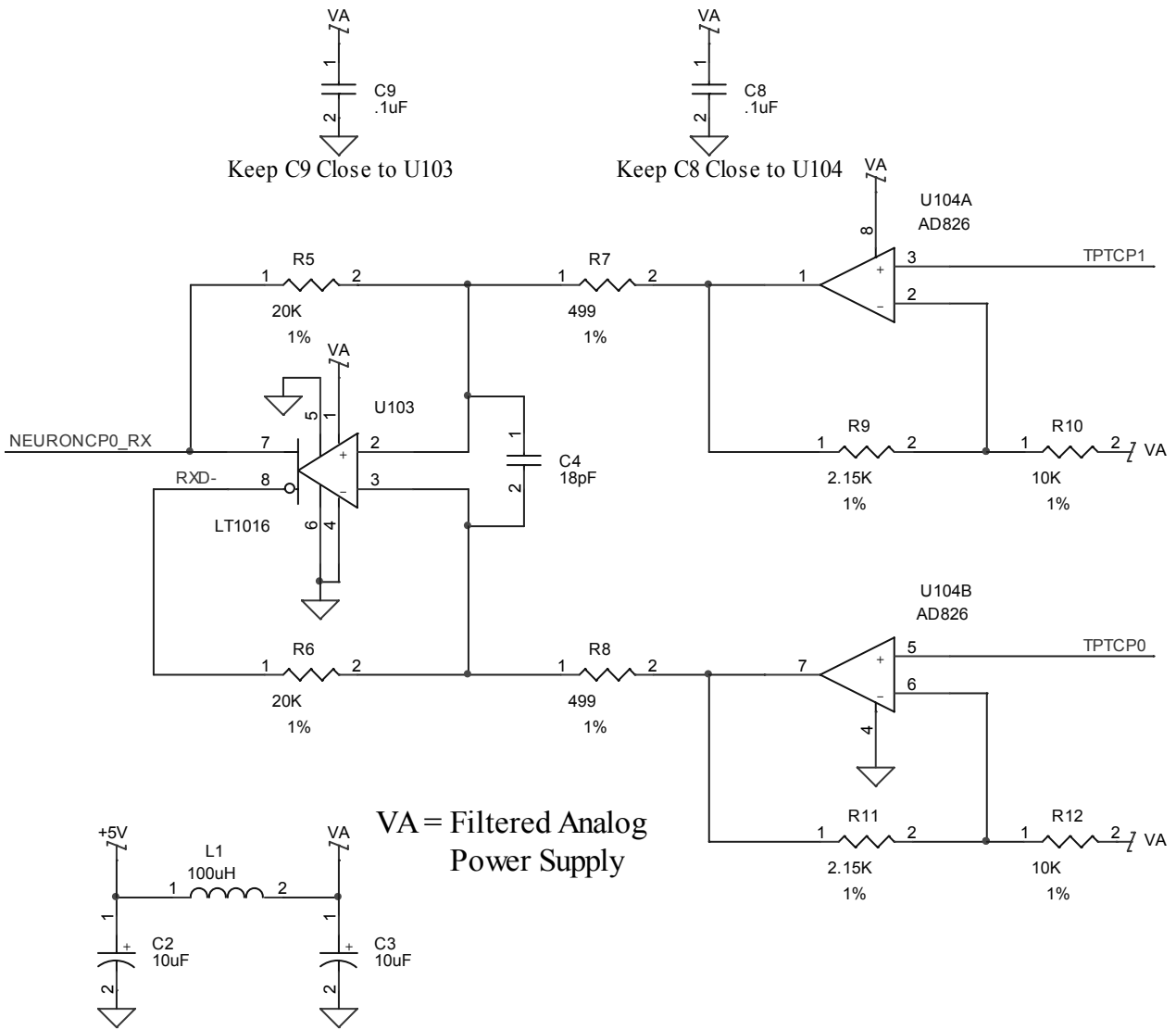
Figure 3. Differential Comparator Circuit
