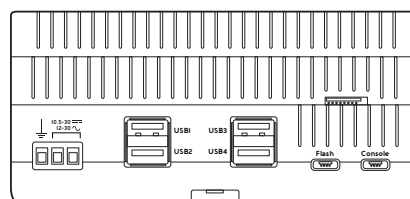
Bottom: Power input terminals, USB ports, flash memory, and console interfaces
